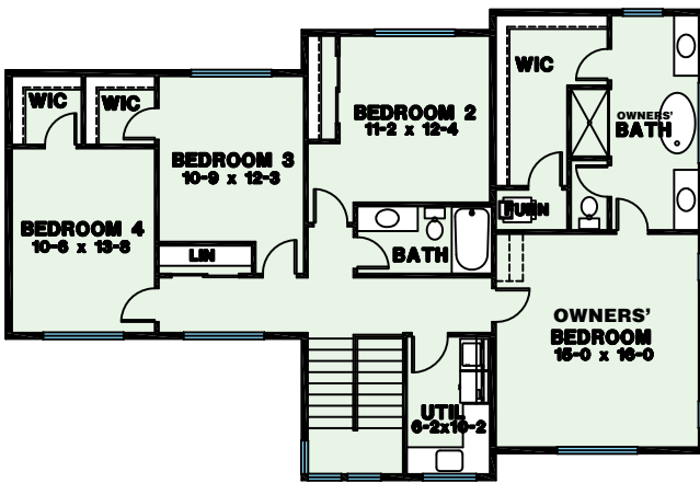
MAIN FLOOR
